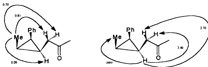
Figure 1. NOE experiment for 5a
