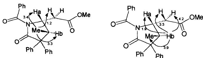
Figure 2. NOE experiment for 9a
